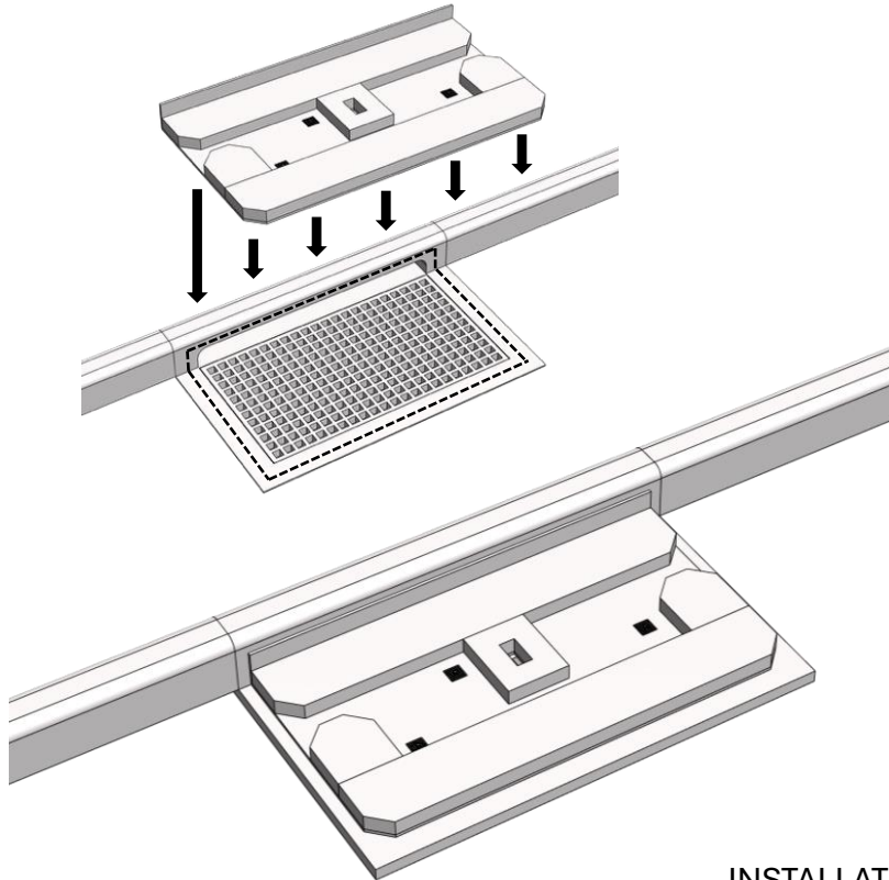
DETAIL A – TYPE-C INLET (SIDEWALL)
